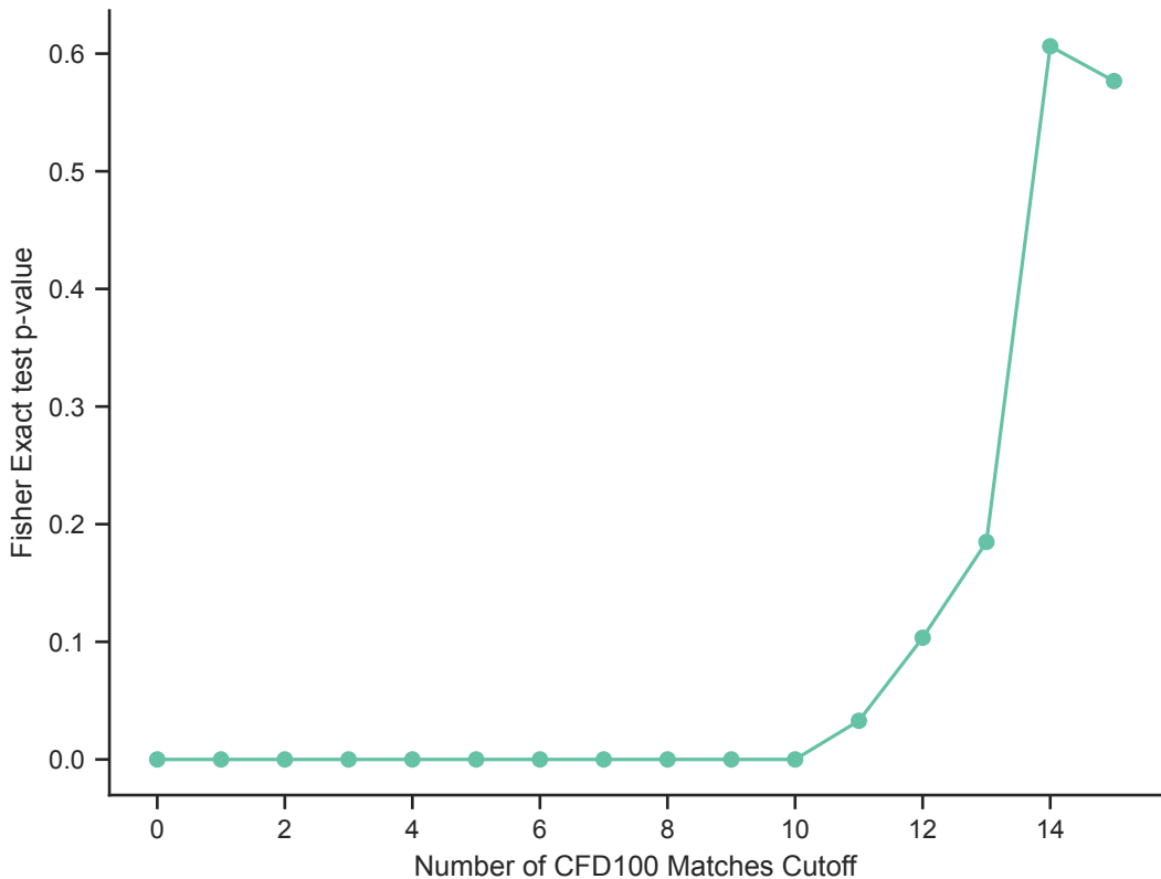
Testing association between having >cutoff CFD100 matches and guide promiscuity (only guides with 0 GGs)
